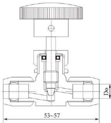
TK12-21 QE-1 气动管路截止阀 TK12-22 QE-2 气动管路三通截止阀 TK12-41 QE-3 气动管路角式截止阀 TK12-21 QE-1 Pneumatic Tube Stop Valve TK12-22 QE-2 Pneumatic Tube Stop Valve TK12-41 QE-3 QE-3 PanPneumatic Tube Stop Valve
