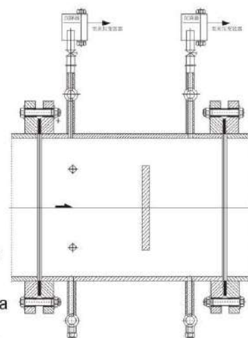
环形孔板 Circular orifice plate
