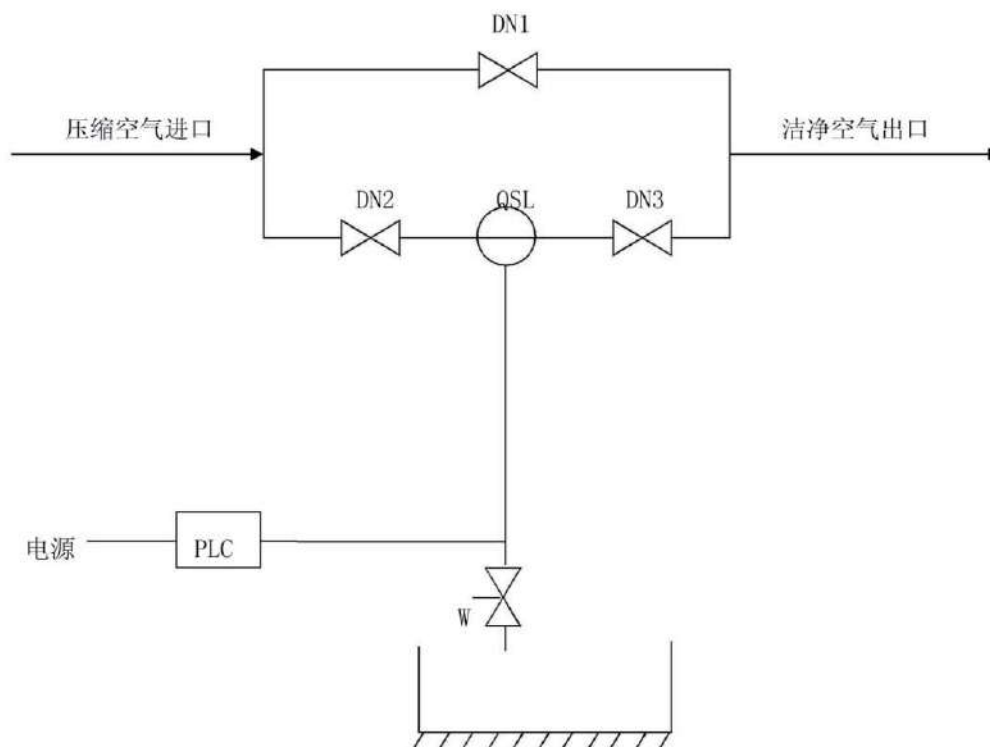
Figure 4.1 installation diagram of tkpsa-t type intelligent air source purification device
