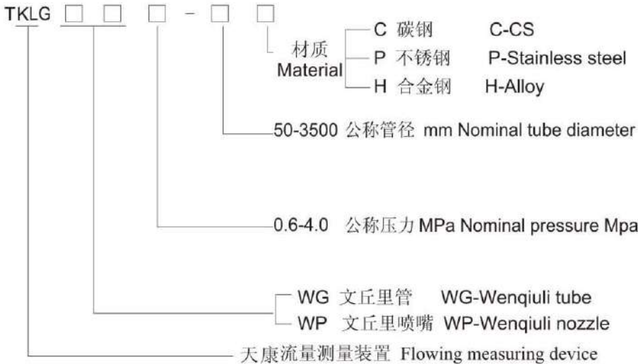
经典文丘里管 Traditional Wenqiuli Nozzle
