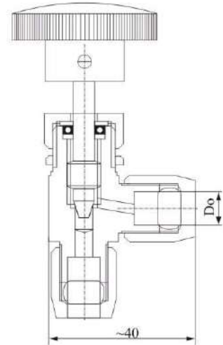
TK12-21 QE-1 气动管路截止阀 TK12-22 QE-2 气动管路三通截止阀 TK12-41 QE-3 气动管路角式截止阀 TK12-21 QE-1 Pneumatic Tube Stop Valve TK12-22 QE-2 Pneumatic Tube Stop Valve TK12-41 QE-3 QE-3 PanPneumatic Tube Stop Valve
