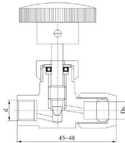
TK6-4 QJ-3A 型气动管路截止阀 TK6-4 QJ-3A Pneumatic Tube Stop Valve
