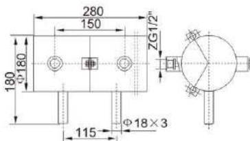
TKF1-21 冷凝器(L1-2.5 型) TKF1-21 Condenser
