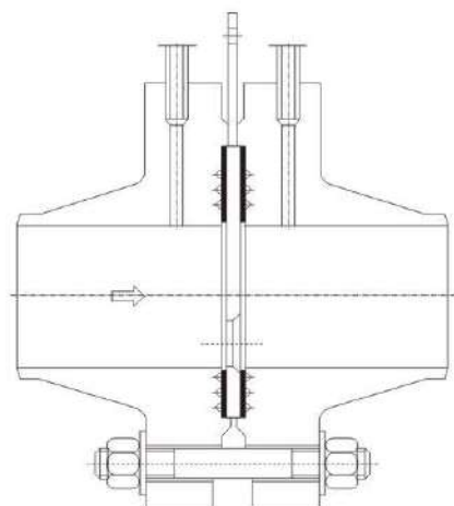
偏心孔板 Eccentric orifice plate
