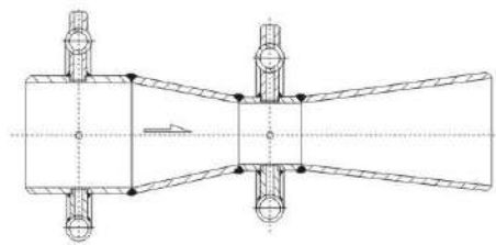
经典文丘里管 Traditional Wenqiuli Nozzle
