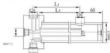
TKF1-15 双室平衡容器 TKF1-15 Two chamber balance vessel
