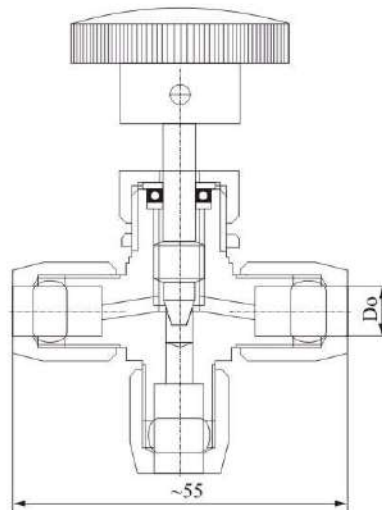
TK12-21 QE-1 气动管路截止阀 TK12-22 QE-2 气动管路三通截止阀 TK12-41 QE-3 气动管路角式截止阀 TK12-21 QE-1 Pneumatic Tube Stop Valve TK12-22 QE-2 Pneumatic Tube Stop Valve TK12-41 QE-3 QE-3 PanPneumatic Tube Stop Valve
