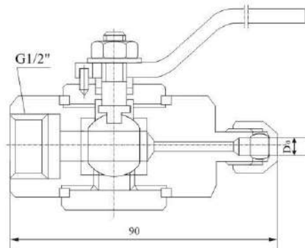
TK9-4 QG.QY1 型气源球阀 TK9-4 QG.QY1 Gas Supply Ball Valve
